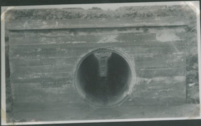
HEADING WALL IMMEDIATELY AFTER REMOVAL OF SHUTTERING.
